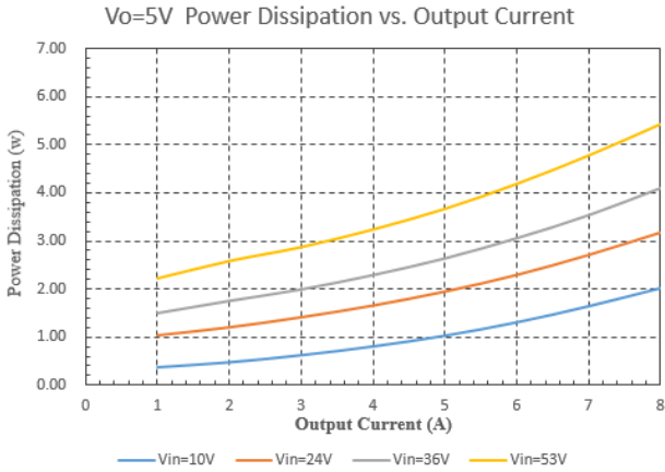
Figure 7: Power Dissipation vs. Output Current(Vo=5V)
