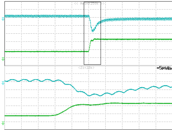
Figure 17: Transient Response
