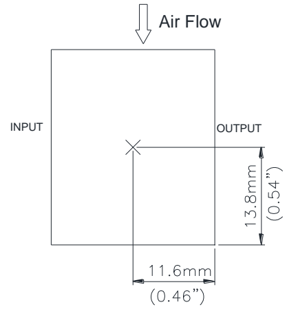
Figure 32: * Hot spot temperature measured point. The allowed maximum hot spot temperature is defined at 115°C.
